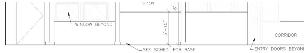
ELEVATIONS - B CASHIERS 1/4" = 1'-0"
